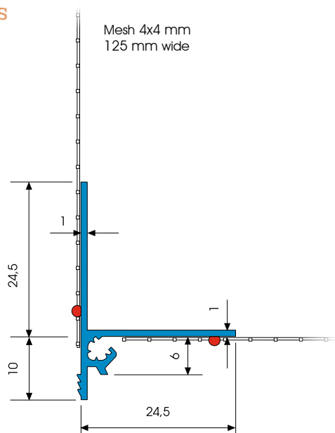
Sectional drawing in mm
