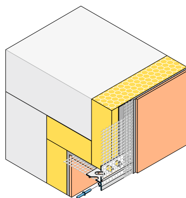
Application drawing
